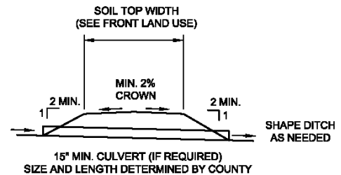
SECTION VIEW
