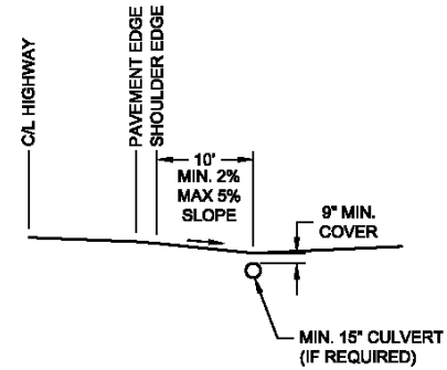
PROFILE VIEW
